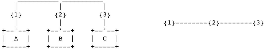
Figure 12: Standard Single Interface Topology (Left), and Corresponding NHDP Representation (Right)
